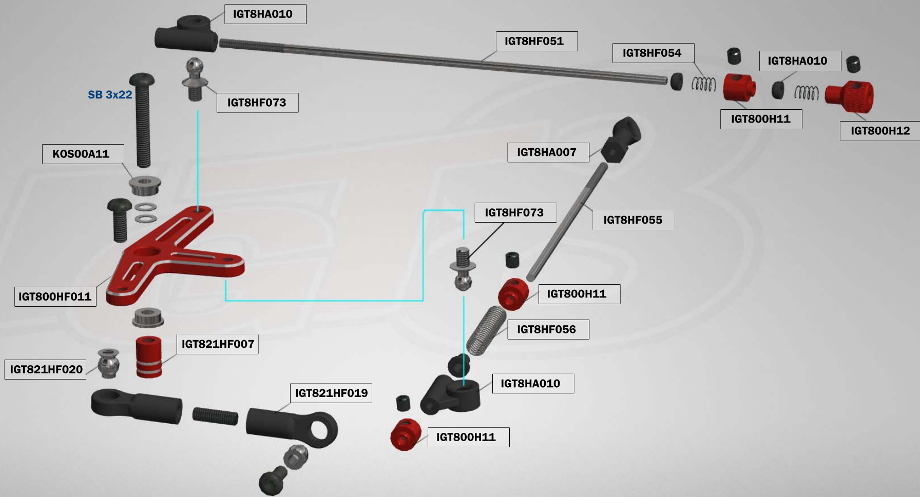
BELLCRANK - EXPLODED VIEW
