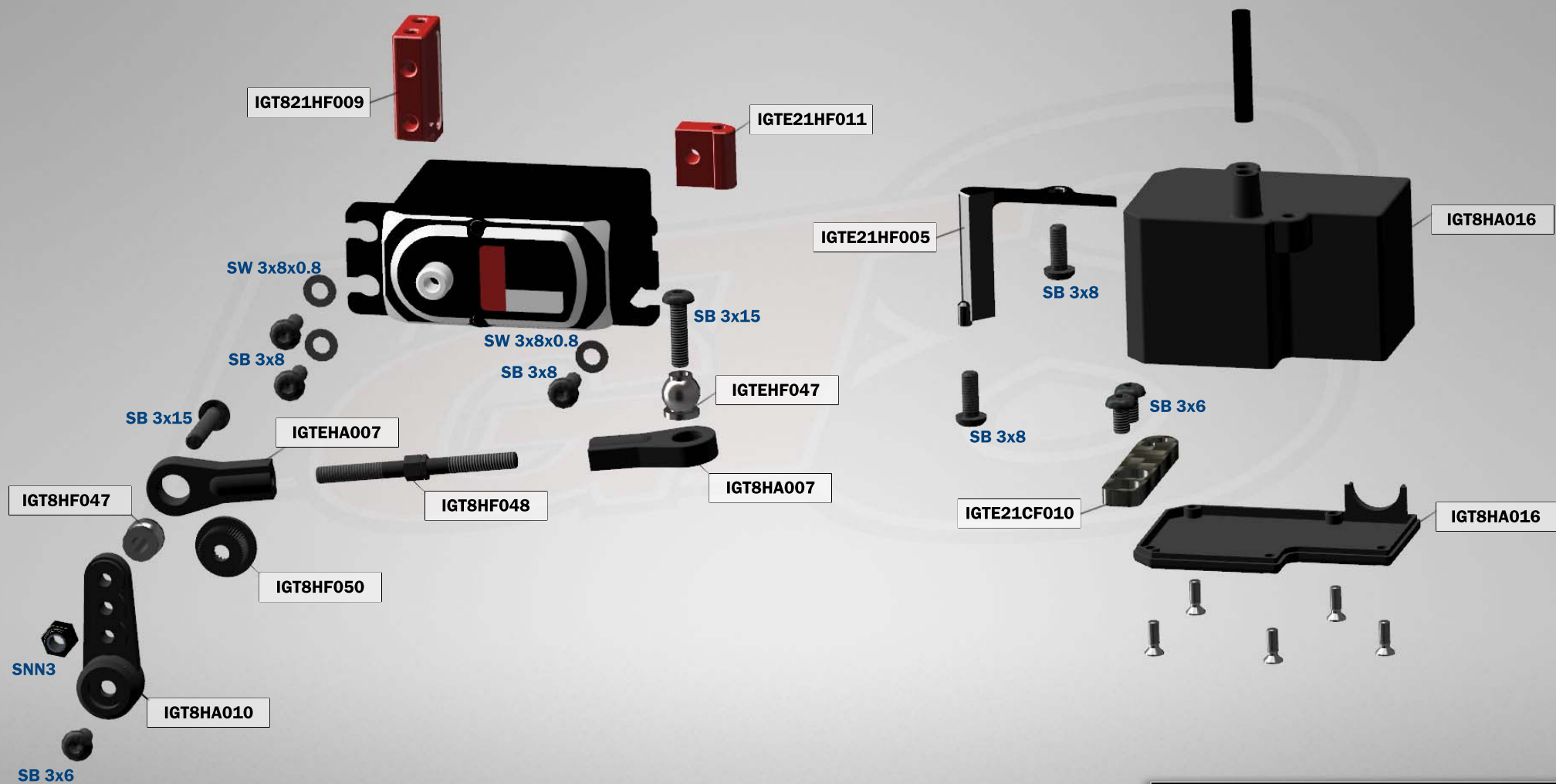
STEERING SERVO & RADIO BOX- EXPLODED VIEW
